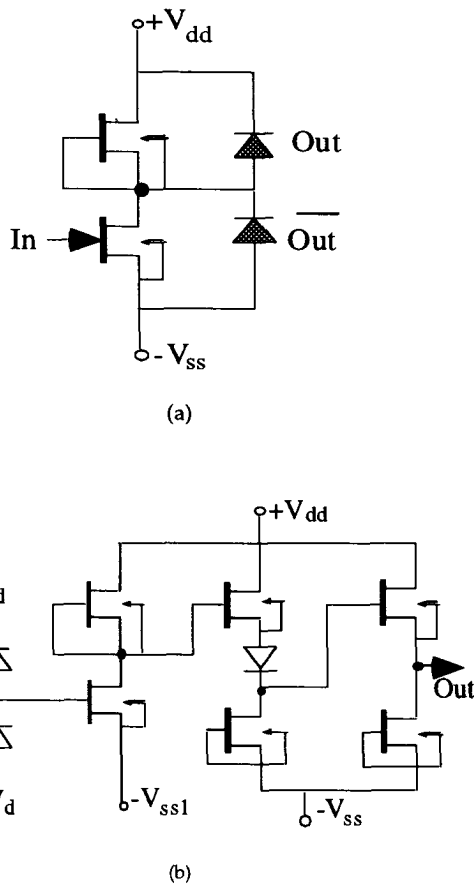
Figure 1: (a) Transmitter circuit, (b) Receiver circuit.
