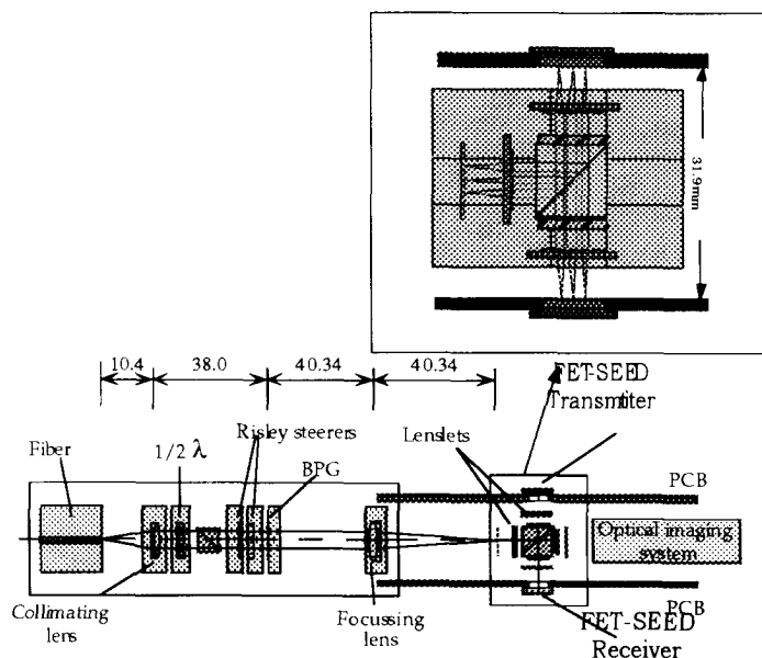
Figure 2a: Optical system layout.
