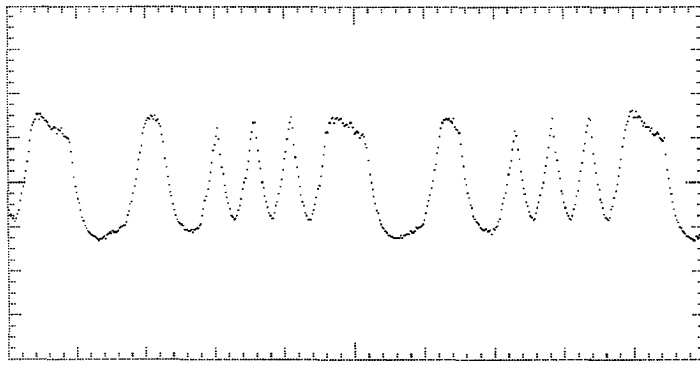
Figure 4: Super Pixel output at 25 MBits/sec.
